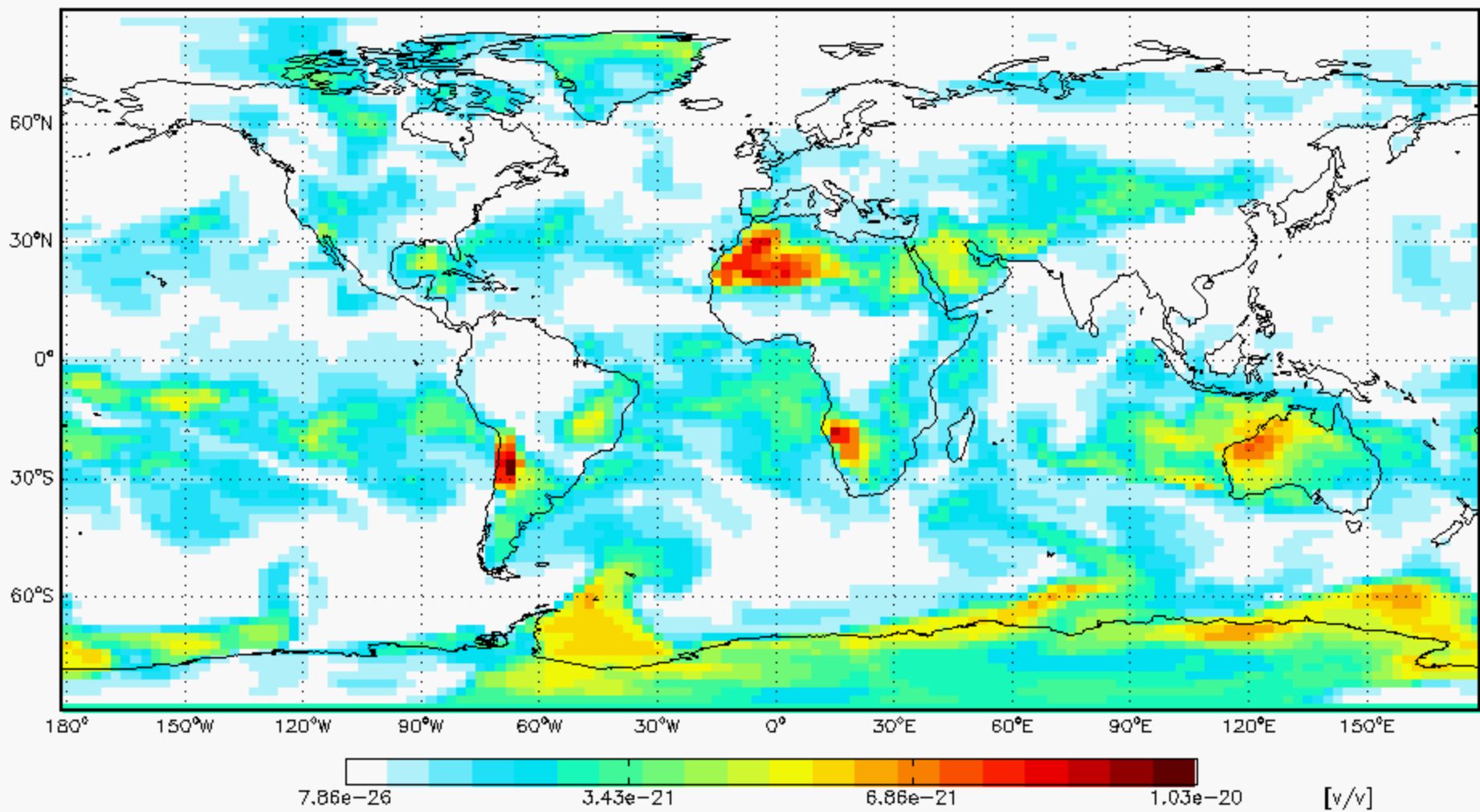
GEOS5 47L OPOG 2 090801 at 00:00 GMT L=1 (0.1 km)
