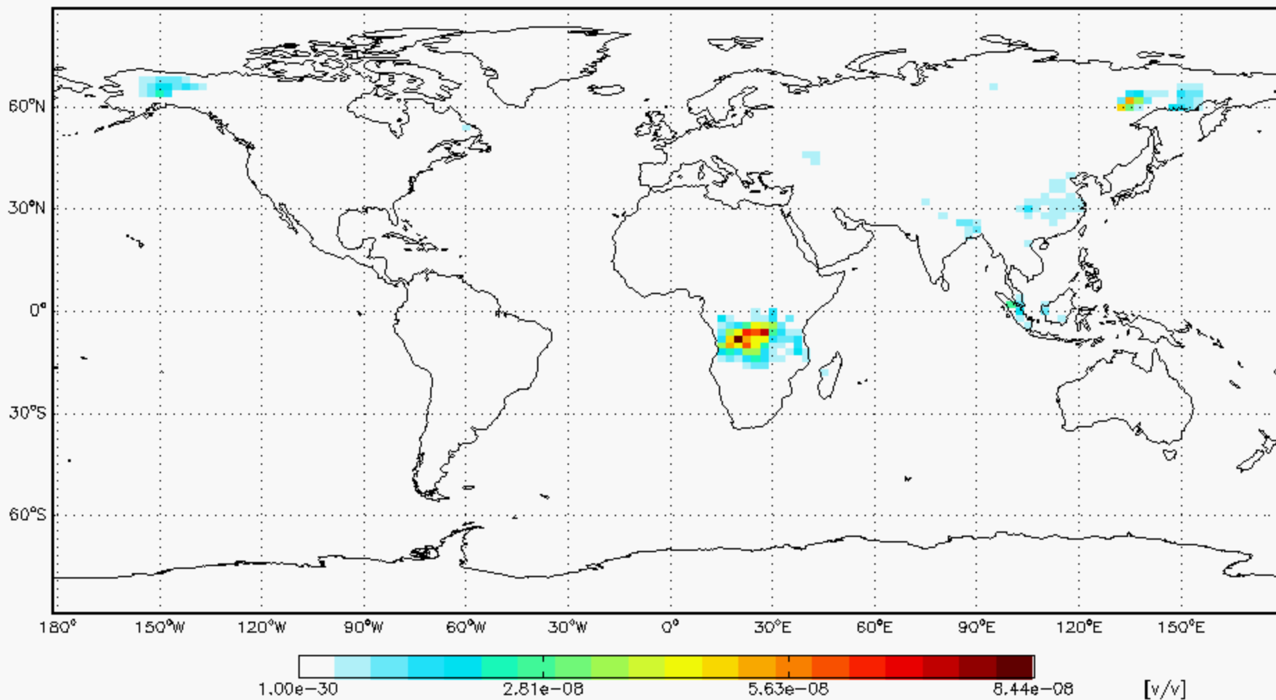
GEOS5 47L OCPO 090801 at 00:00 GMT L=1 (0.1 km)
