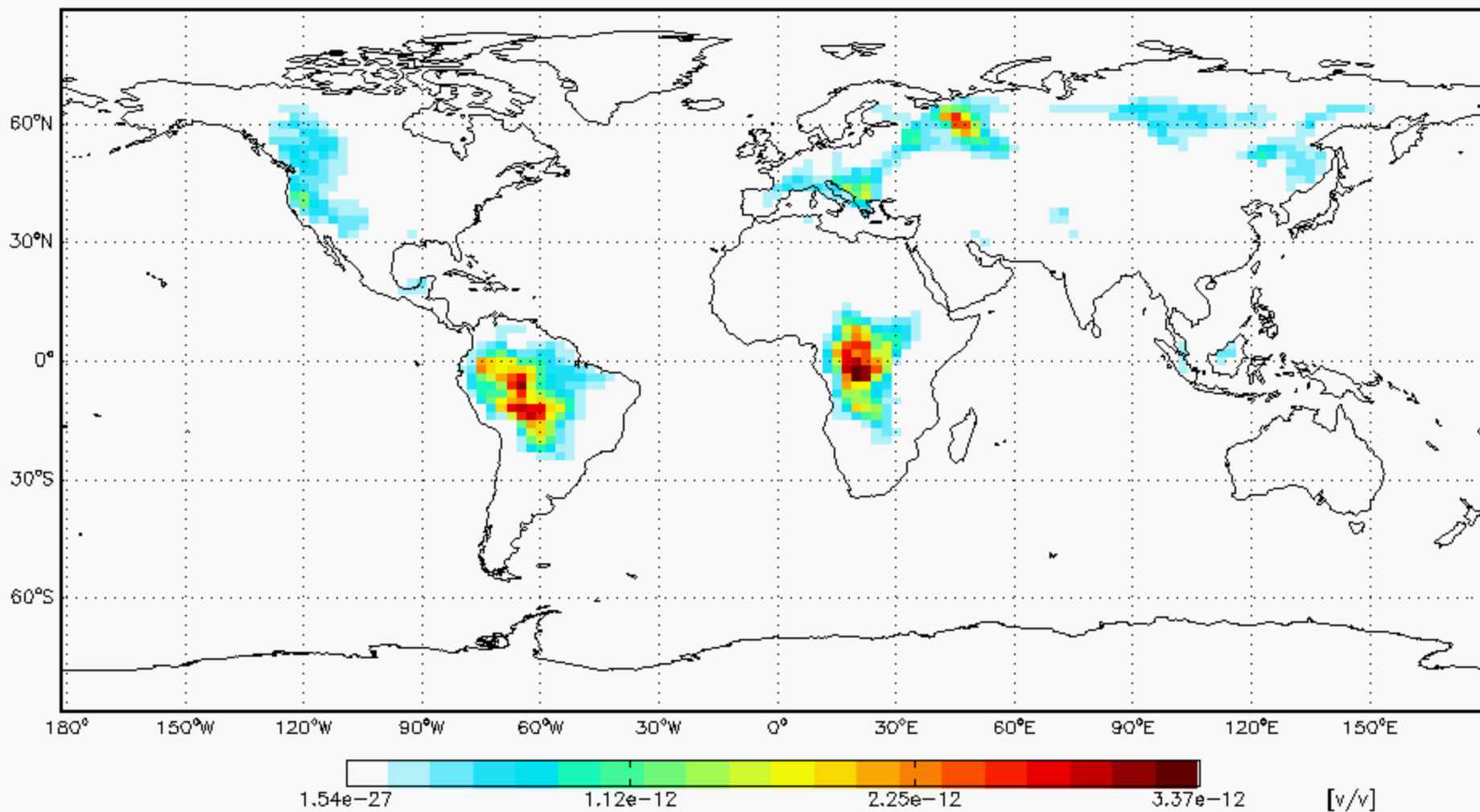
GEOS5 47L OPOA, 090801 at 00:00 GMT L=1 (0.1 km)
