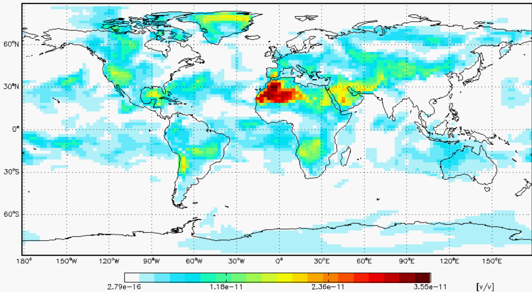
GEOS5 47L OPOG 1 090801 at 00:00 GMT L=1 (0.1 km)
