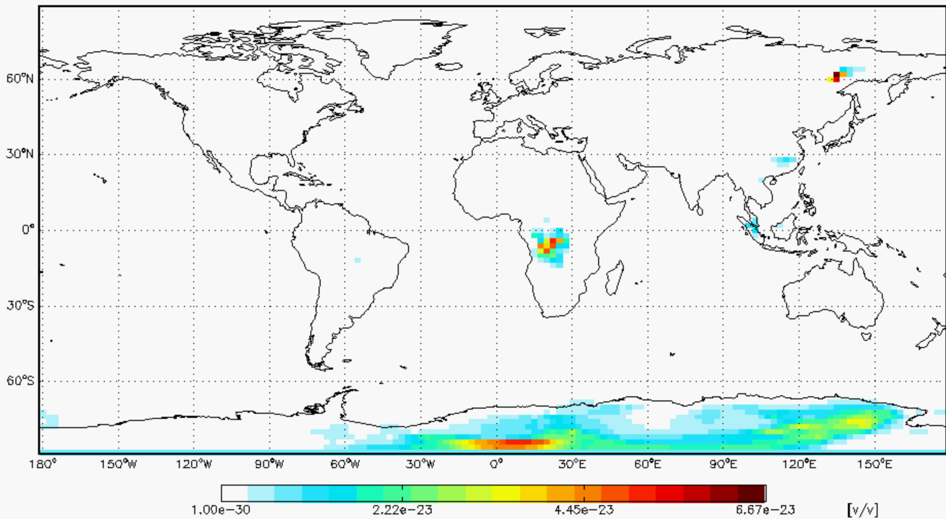
GEOS5 47L POA 2 090801 at 00:00 GMT L=1 (0.1 km)
