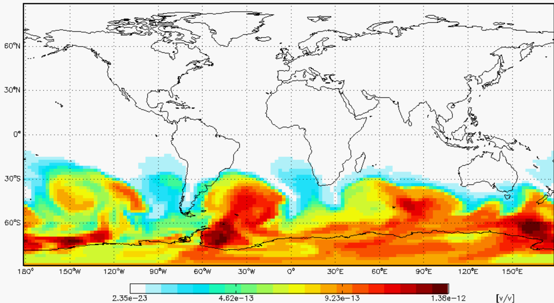
GEOS5 47L POG 1 090801 at 00:00 GMT L=1 (0.1 km)
