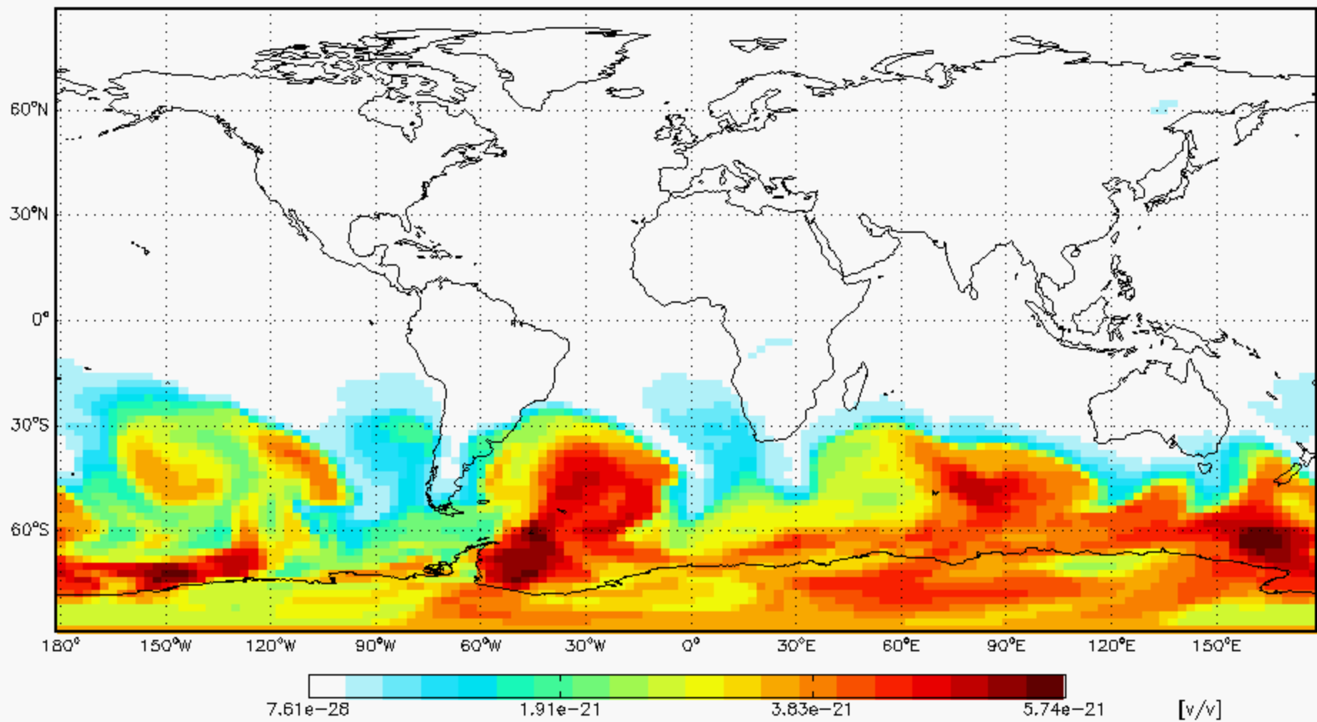
GEOS5 47L POG 2 090801 at 00:00 GMT L=1 (0.1 km)
