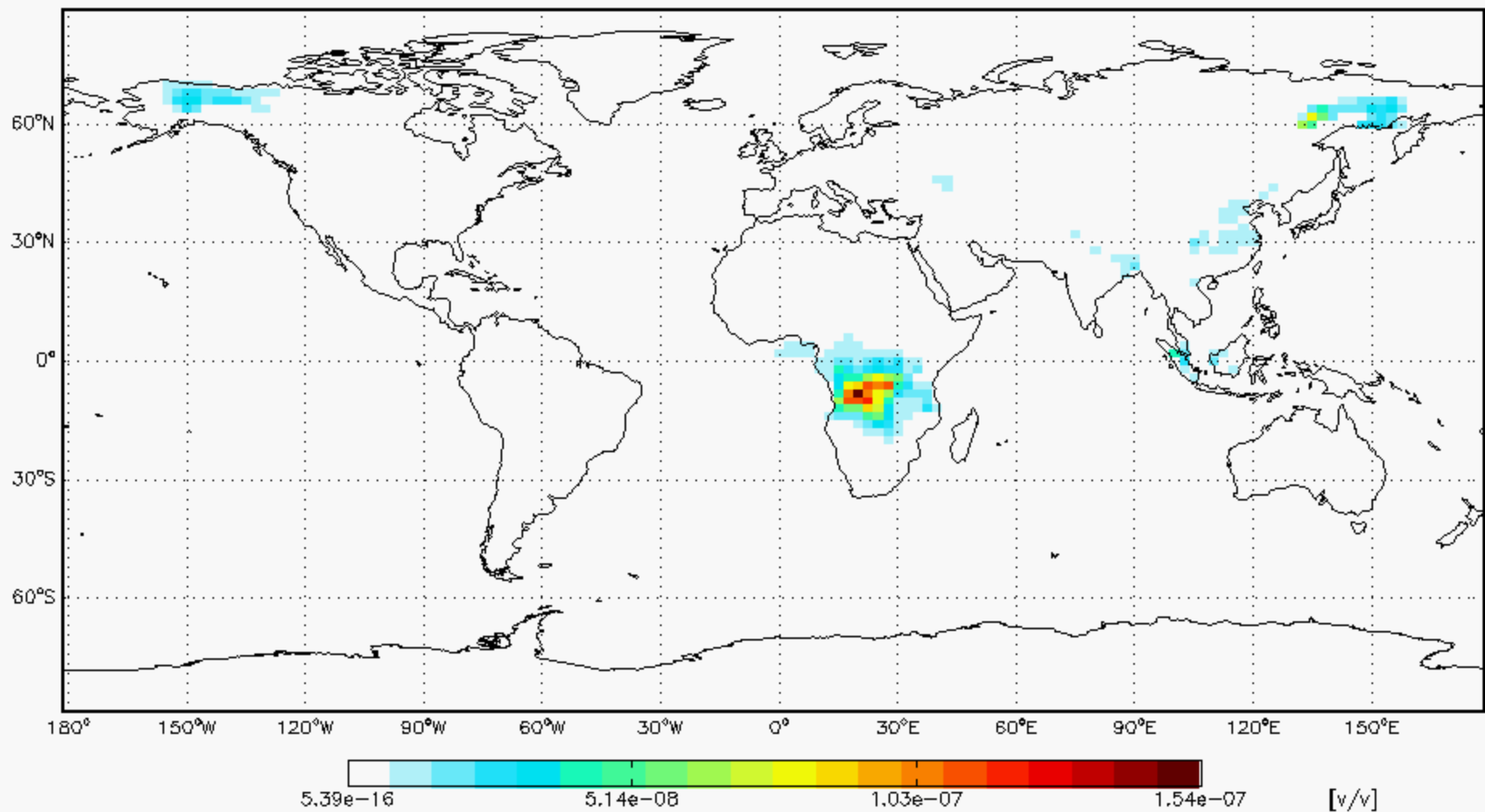
GEOS5 47L OCPI 090801 at 00:00 GMT L=1 (0.1 km)
