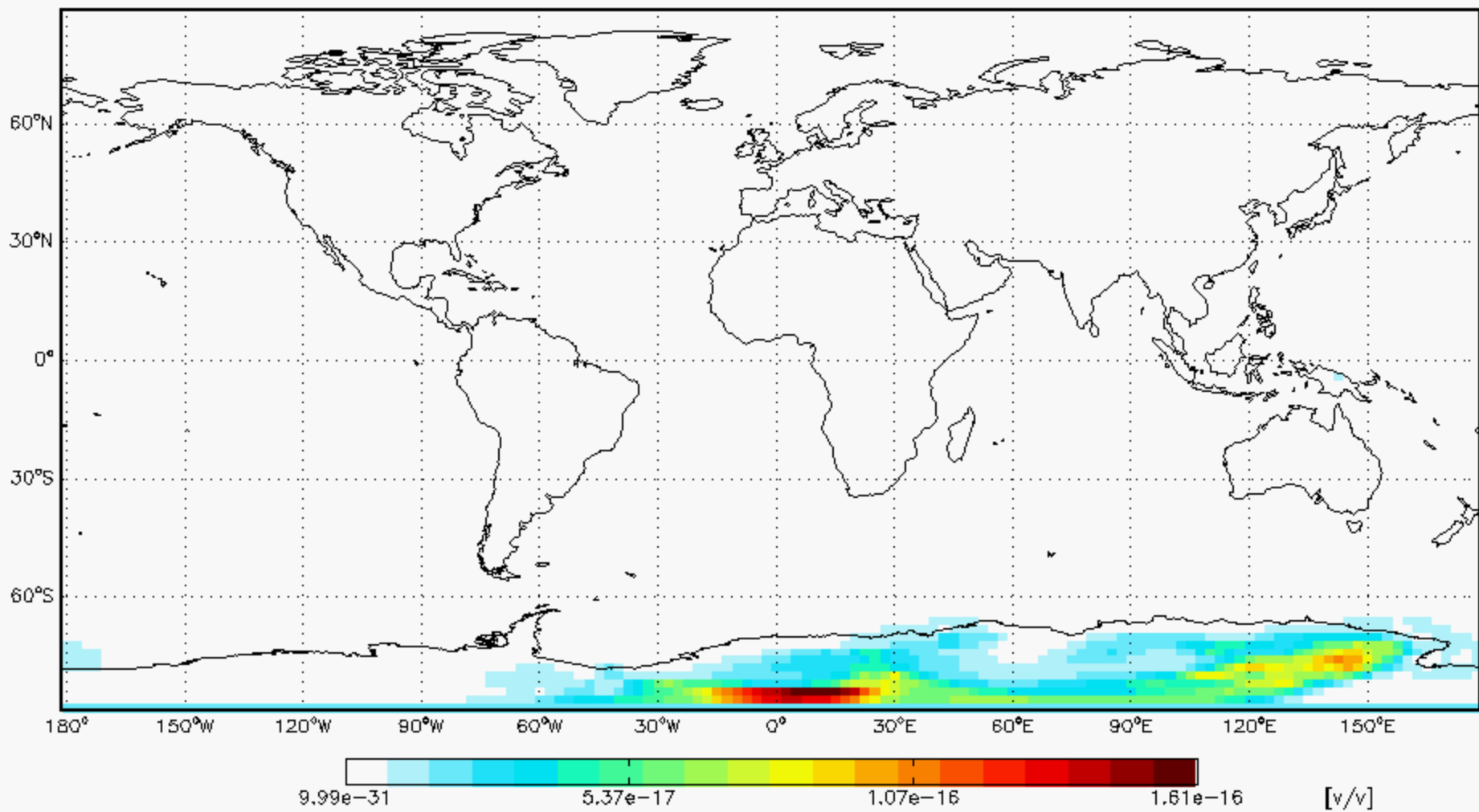
GEOS5 47L POA 1 090801 at 00:00 GMT L=1 (0.1 km)
