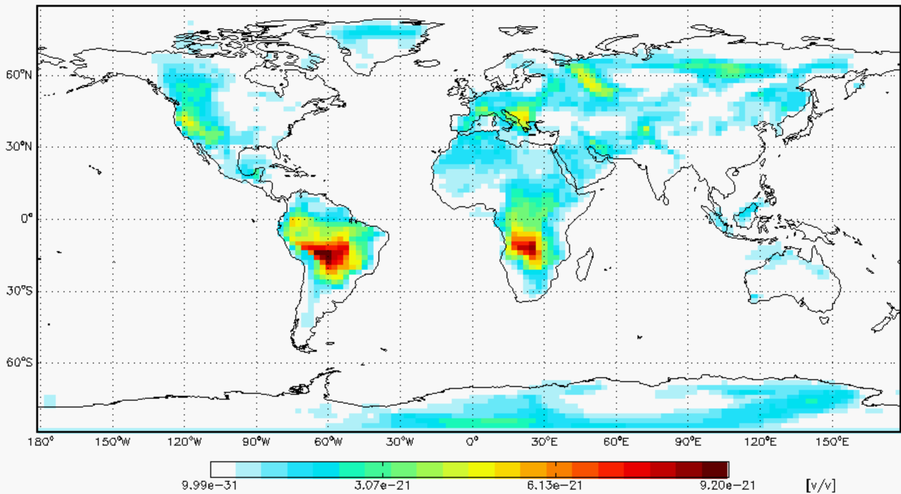
GEOS5 47L OPOA 2 090801 at 00:00 GMT L=1 (0.1 km)
