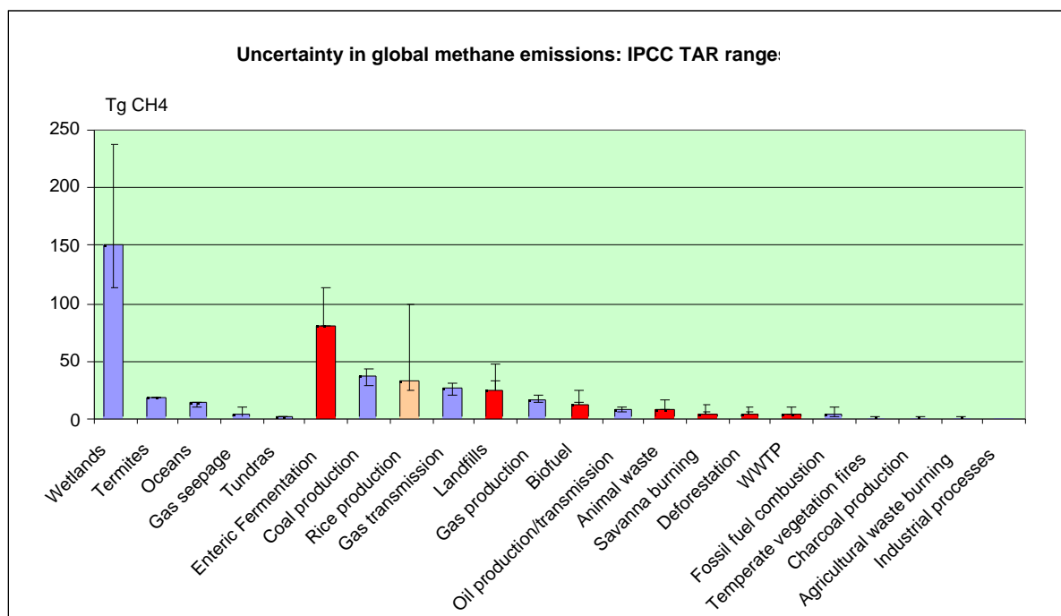
Figure 2. Comparison of uncertainty estimates for major global methane sources (a) using the uncertainty estimates by the EDGAR team and (b) the compilation made for the Third Assessment Report of IPCC Working Group I.
