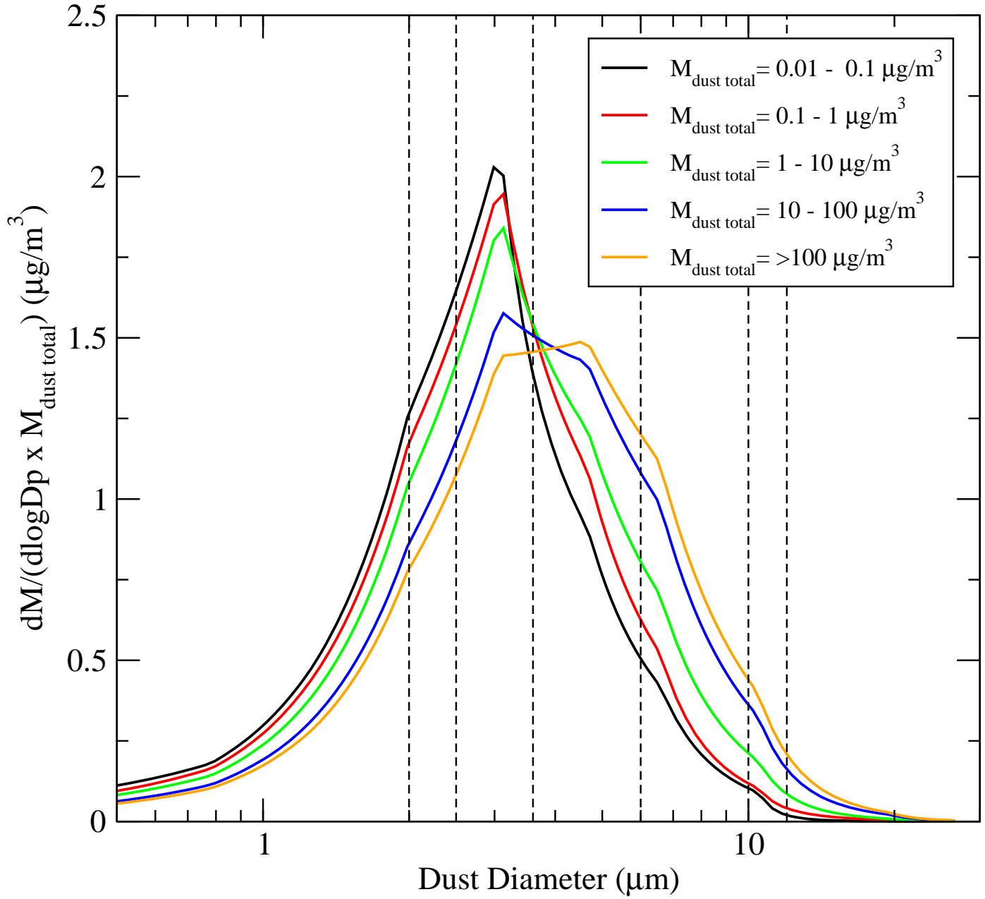
APM-simulated annual mean normalized dust mass size distributions, Beijing
